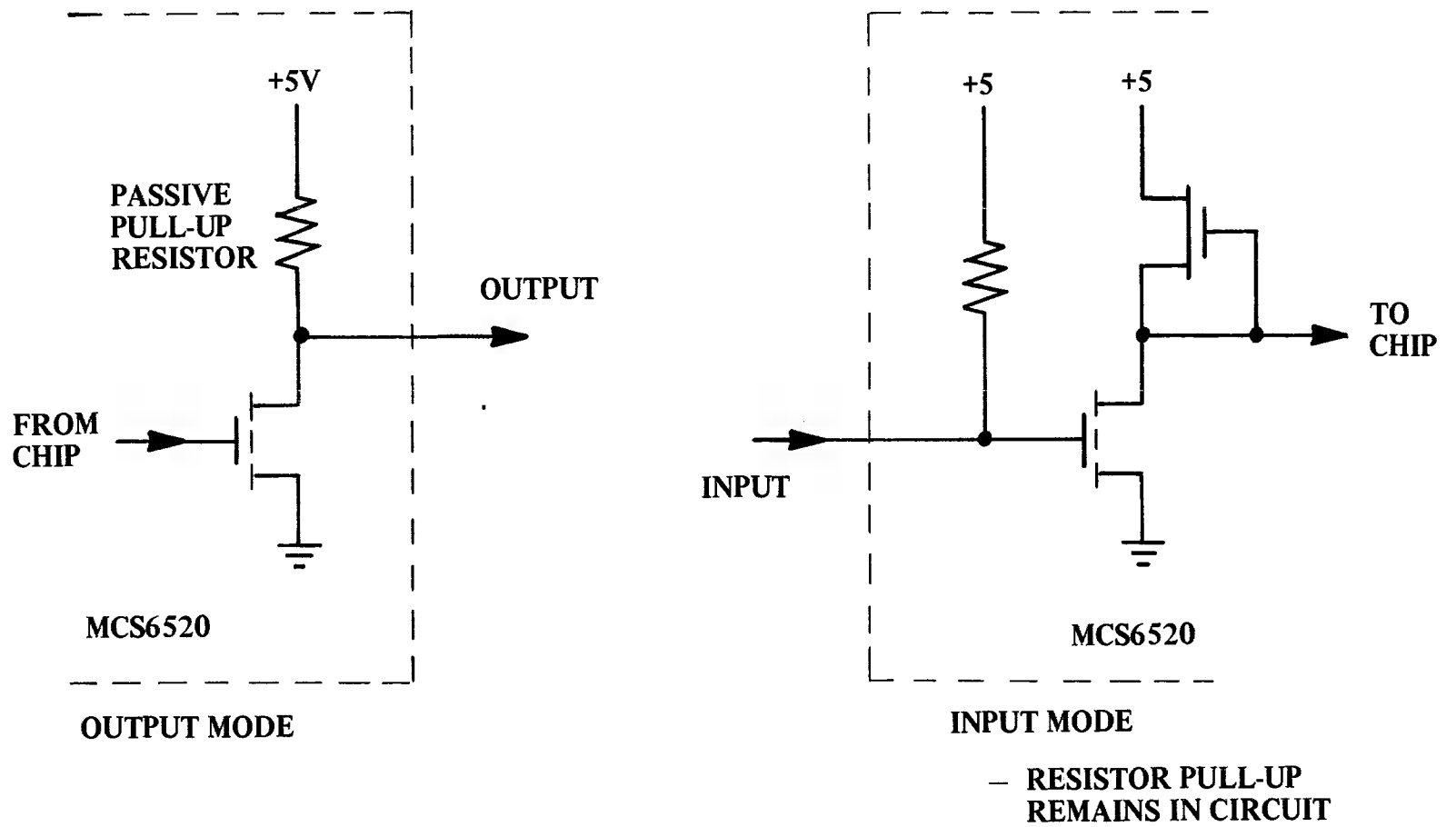
Peripheral I/O Port A Buffer FIGURE 1.28A
